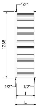
20 ELEMENTS
