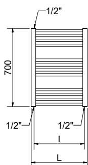
12 ELEMENTS
