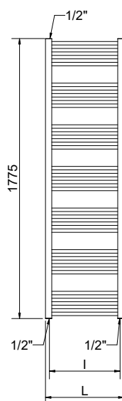
28 ELEMENTS
