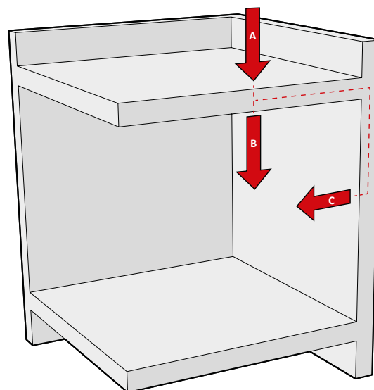
A. Footfall noise B. Direct transmission C. Lateral transmission
