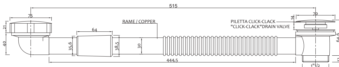
Colonna scarico vasca in ottone/rame click clack Click clack bath tube discharge system in copper/brass
