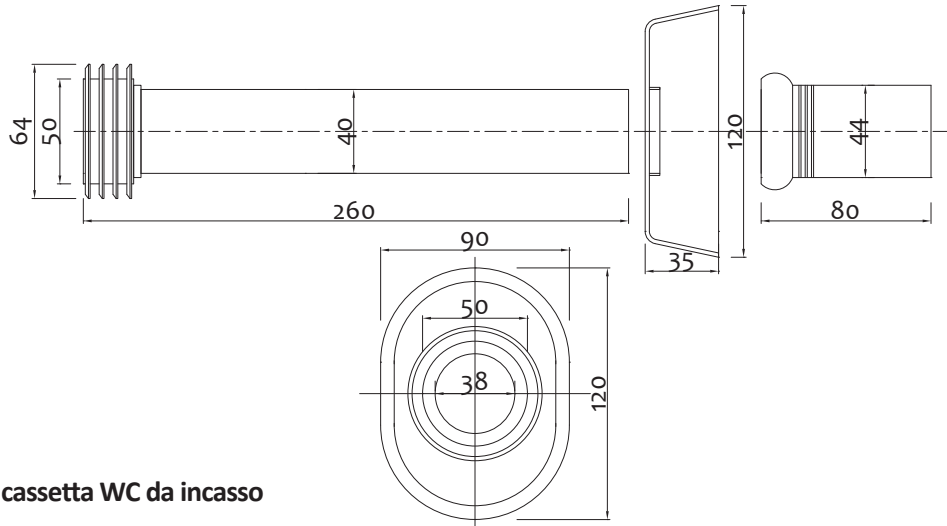
White WC connection pipe for built-in flushing cistern
