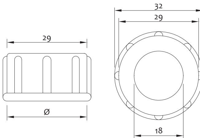
Dado in nylon da 3/4" per tubo carico 3/4" nylon nut for WM inlet pipe
