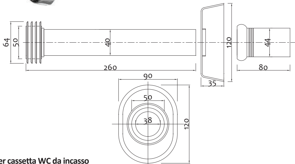
Chromed WC connection pipe for built-in flushing cistern
