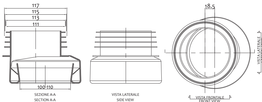
Prolunga WC in PVC eccentrica PVC excentric WC extension
