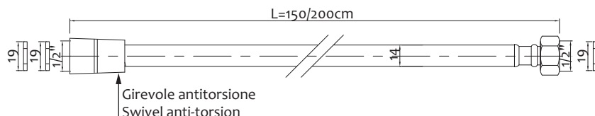
Silver smooth PVC flexible for shower
